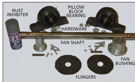
Shaft Kit
