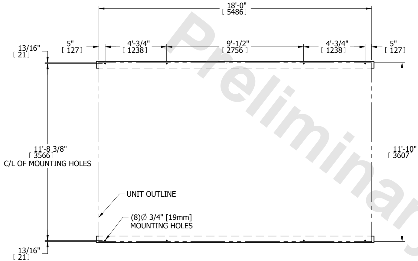
PLAN VIEW
