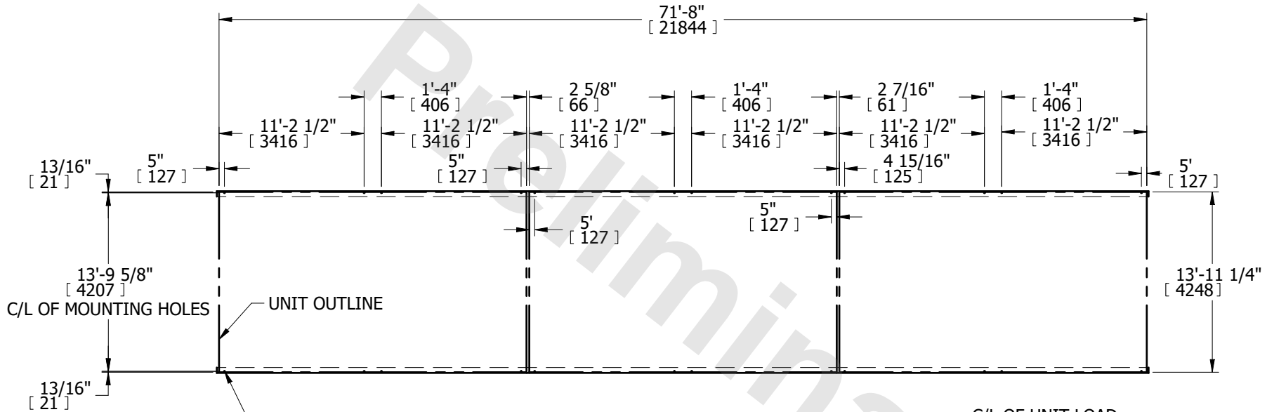
PLAN VIEW
