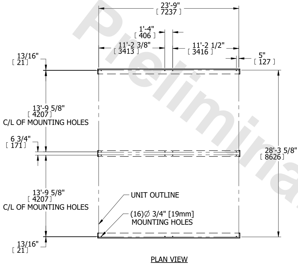
PLAN VIEW
