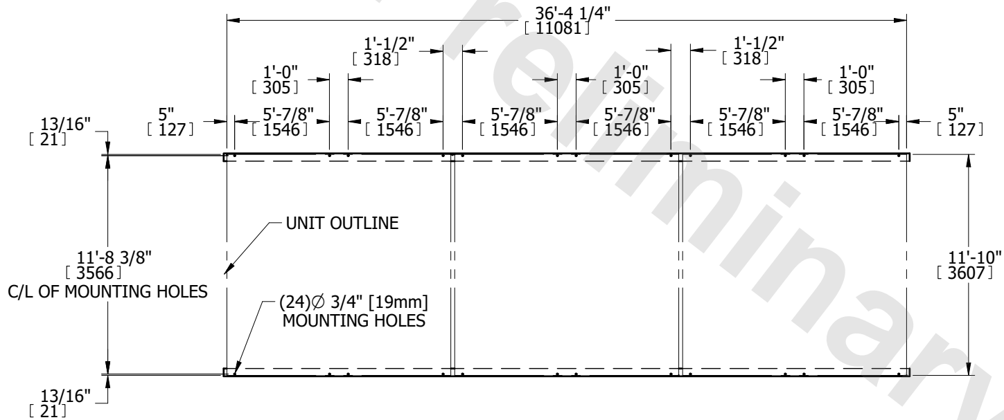
PLAN VIEW
