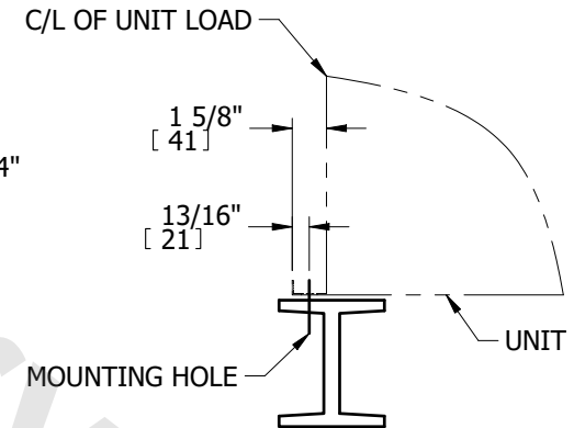
TYPICAL END VIEW
