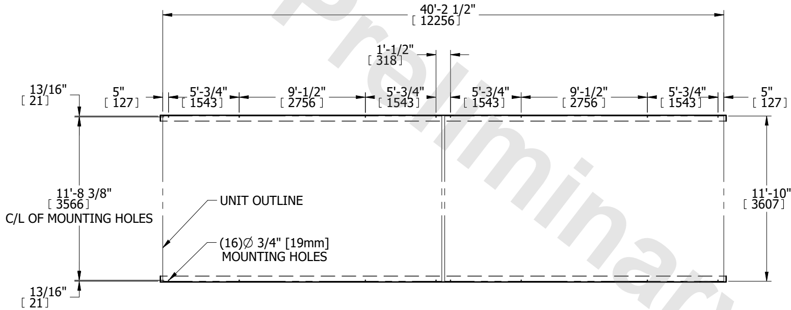
PLAN VIEW
