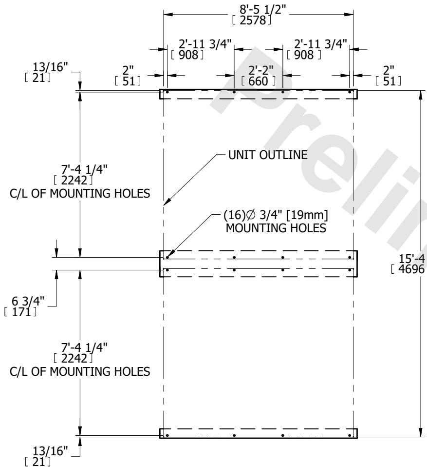
PLAN VIEW
