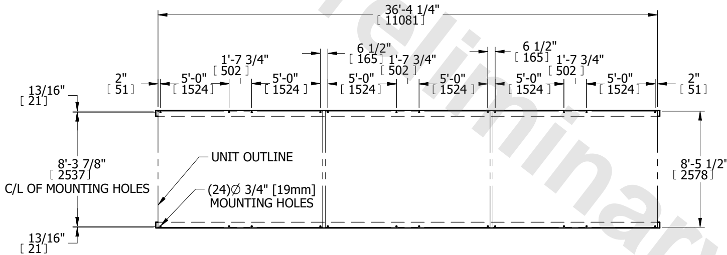
PLAN VIEW
