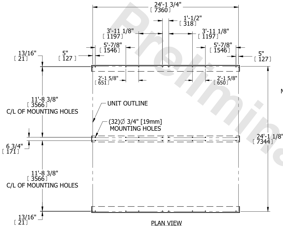
PLAN VIEW
