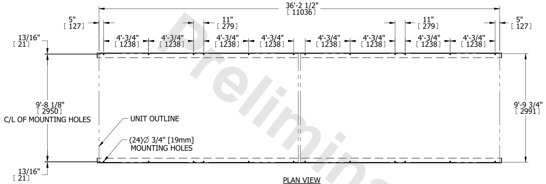
PLAN VIEW
