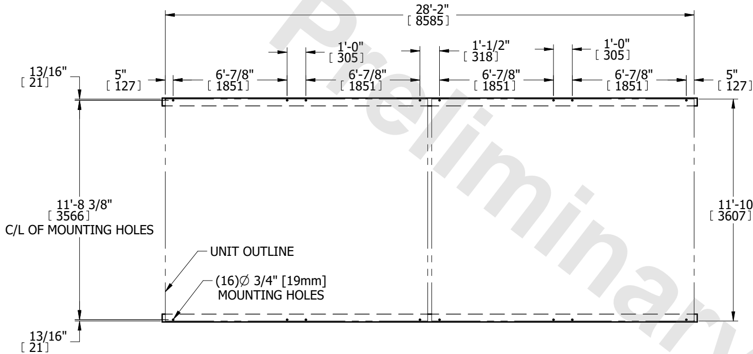
PLAN VIEW
