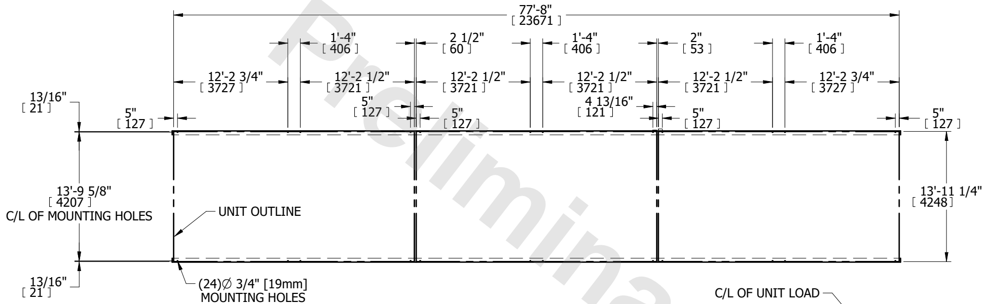
PLAN VIEW
