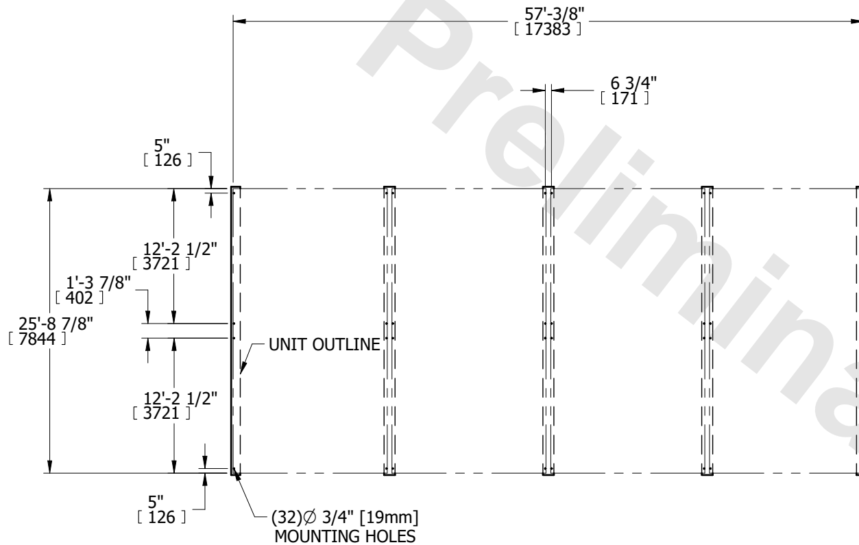
PLAN VIEW
