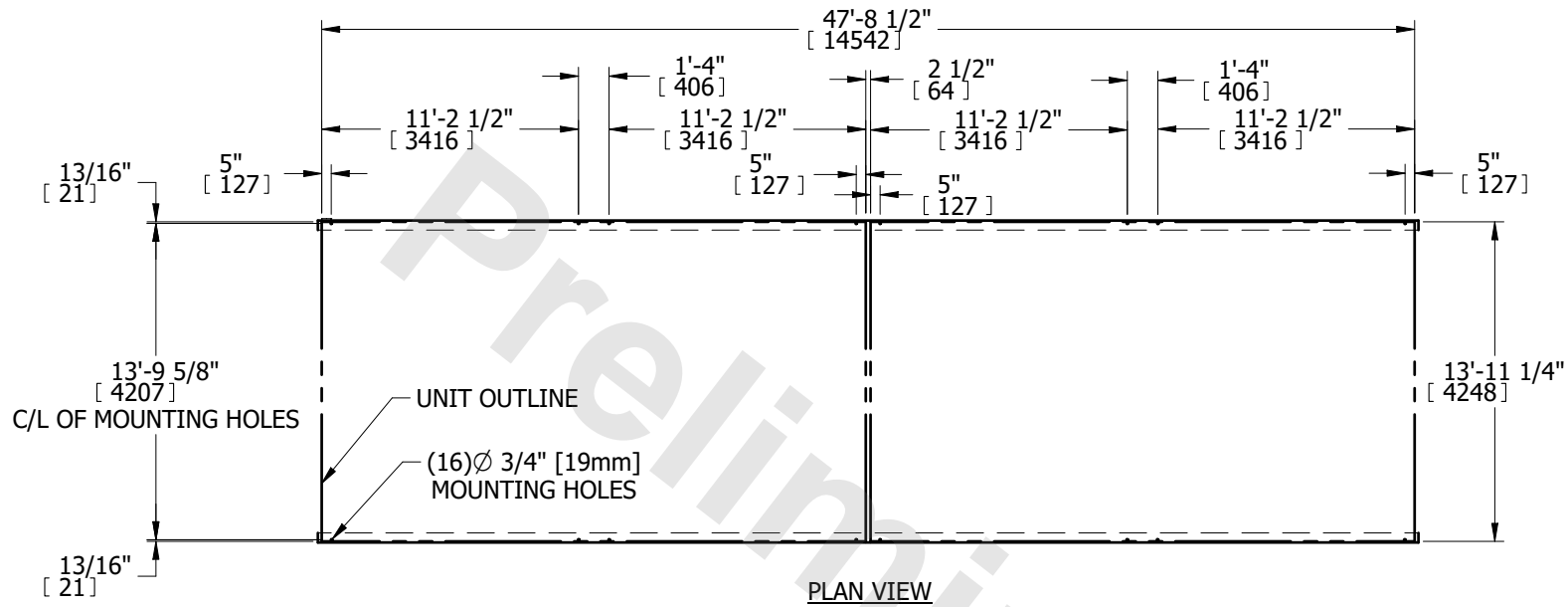
PLAN VIEW
