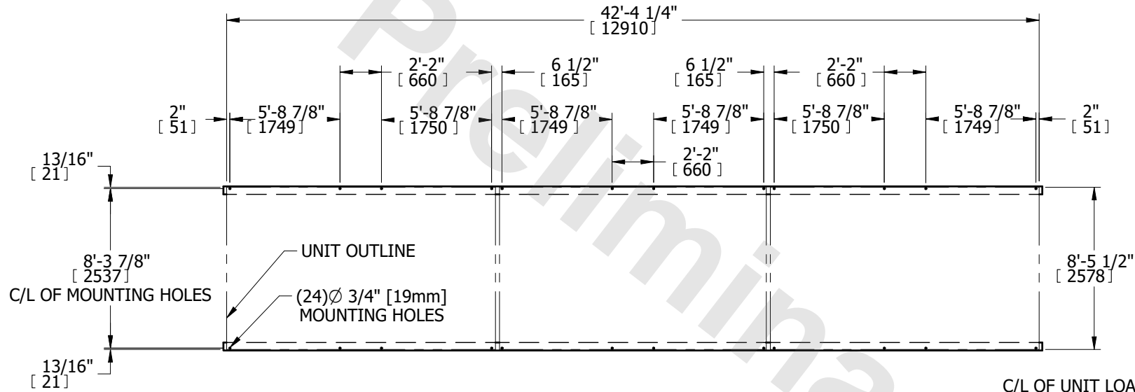
PLAN VIEW
