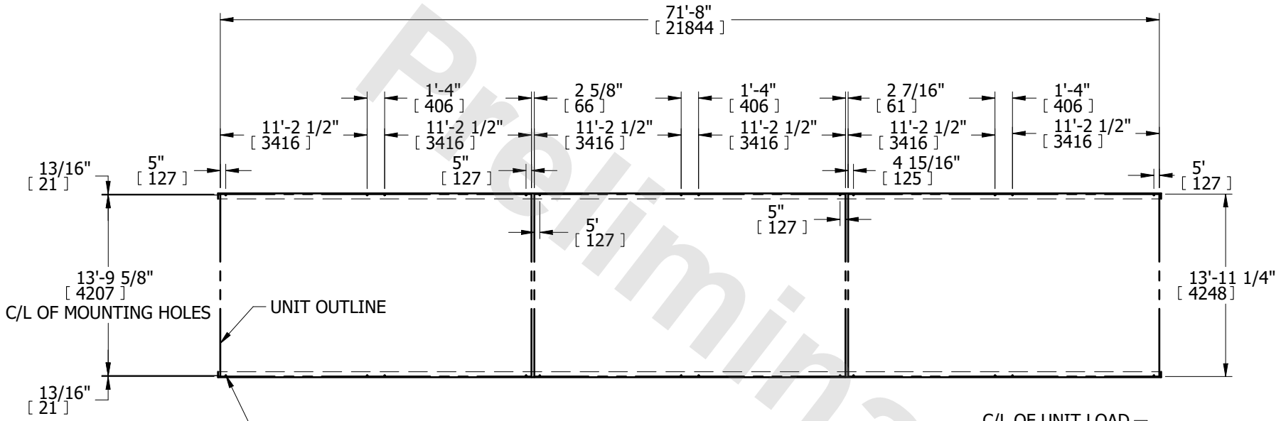
PLAN VIEW
