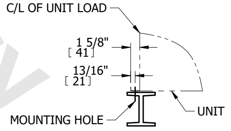
TYPICAL END VIEW
