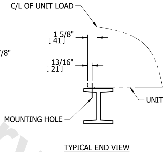
TYPICAL END VIEW
