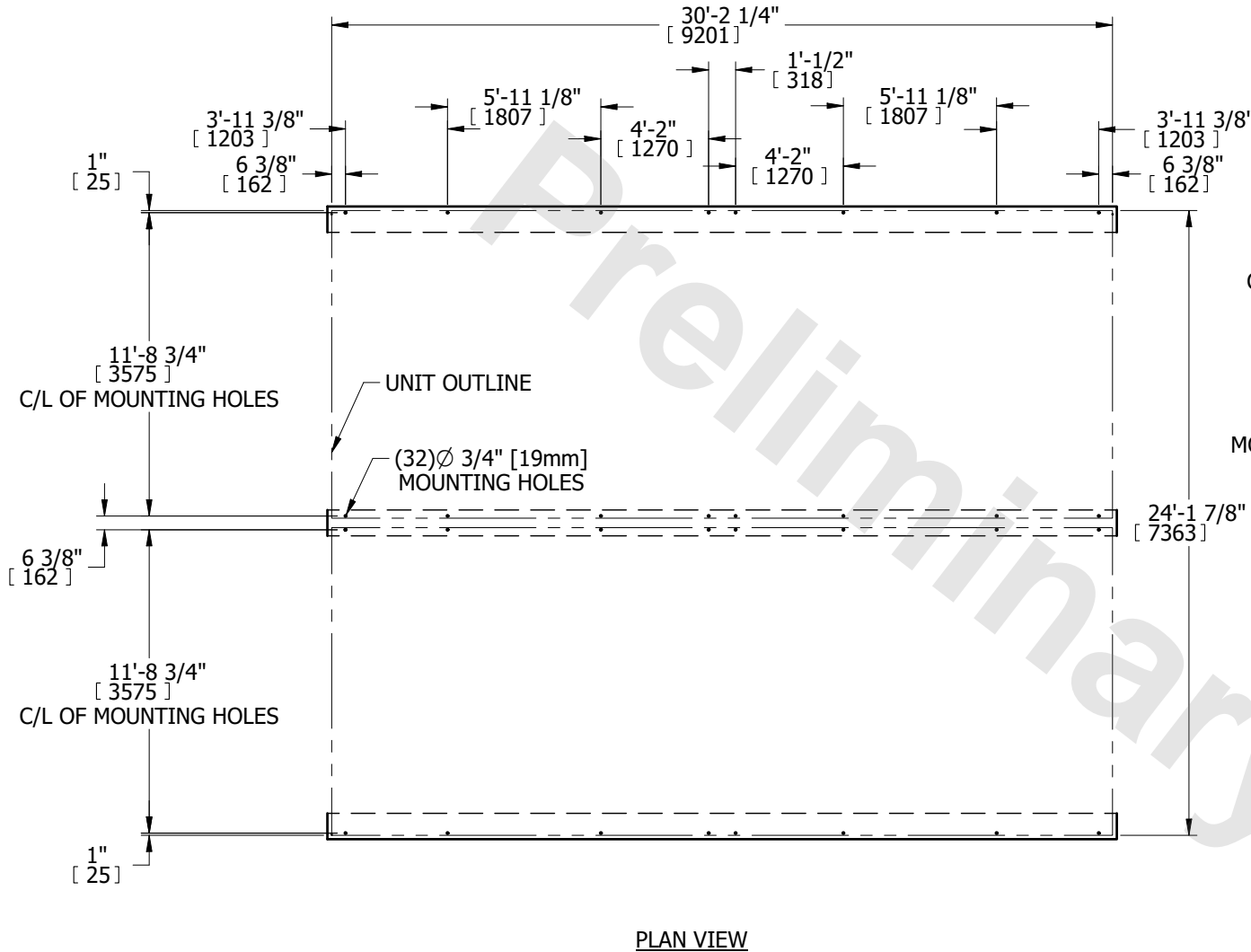
PLAN VIEW
