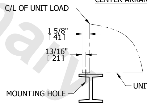
CENTER ARRANGEMENT
