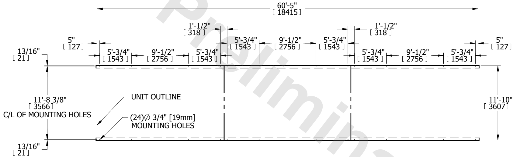
PLAN VIEW
