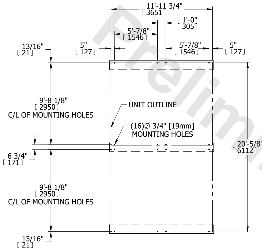
PLAN VIEW
