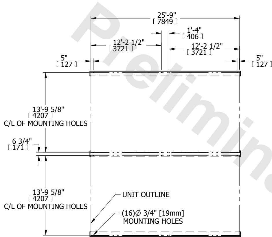
PLAN VIEW
