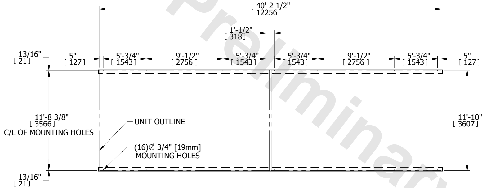
PLAN VIEW
