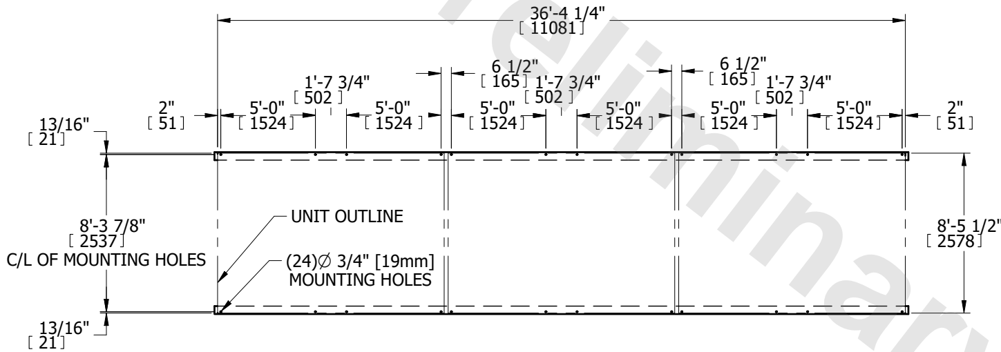
PLAN VIEW
