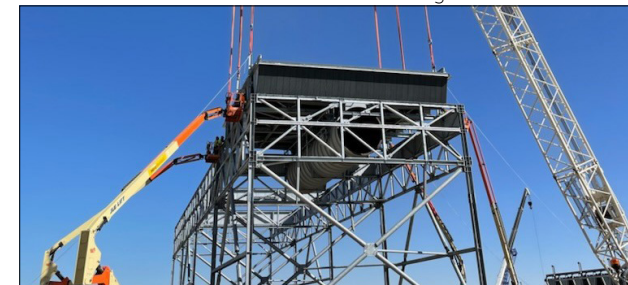
Advanced Technology™ ACC Onsite Modularization
