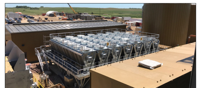
eco-Air Air Cooled Heat Exchangers Factory Assembled Packaged Units Installed on Common Structure
