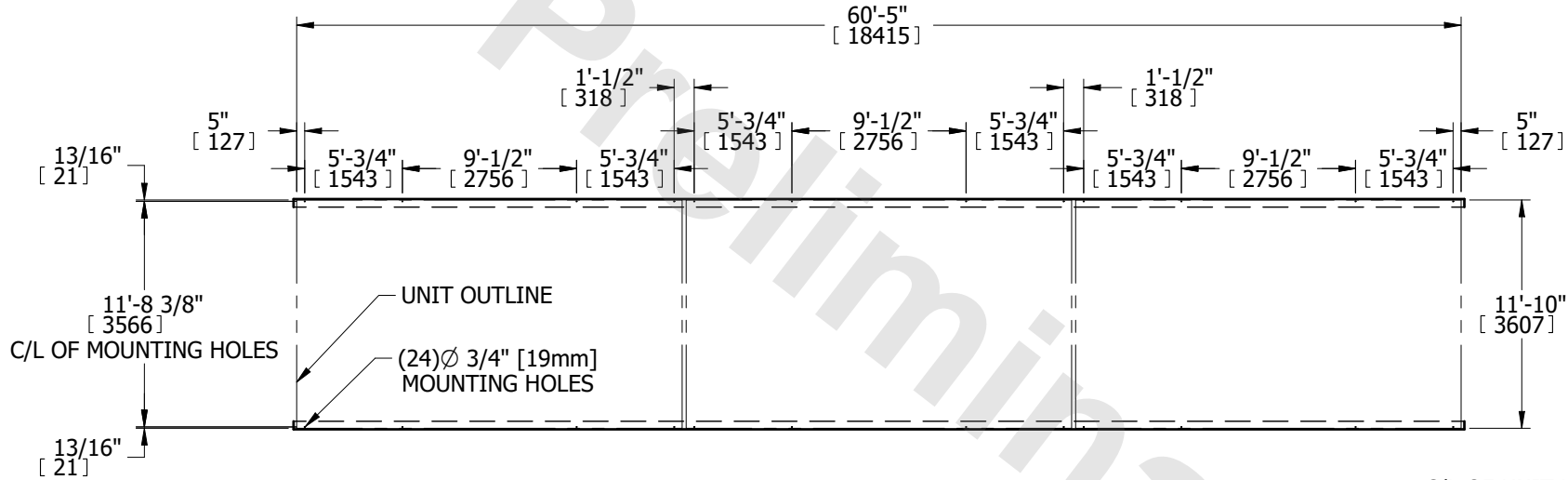
PLAN VIEW
