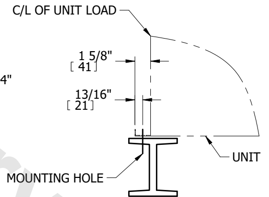
TYPICAL END VIEW
