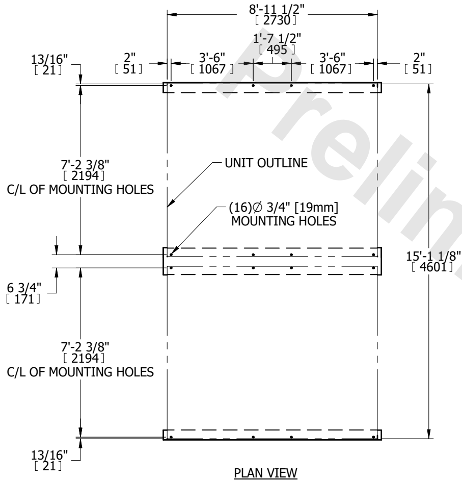
PLAN VIEW
