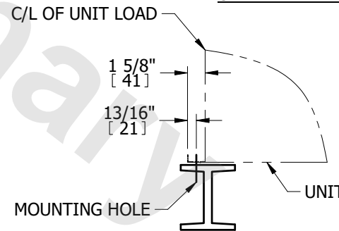
CENTER ARRANGEMENT
