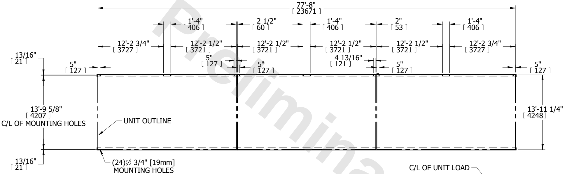
PLAN VIEW
