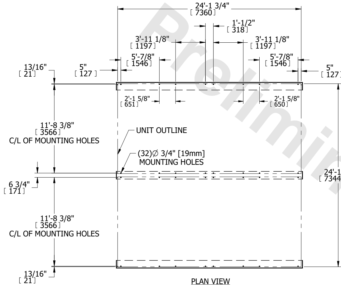
PLAN VIEW
