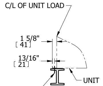
TYPICAL END VIEW
