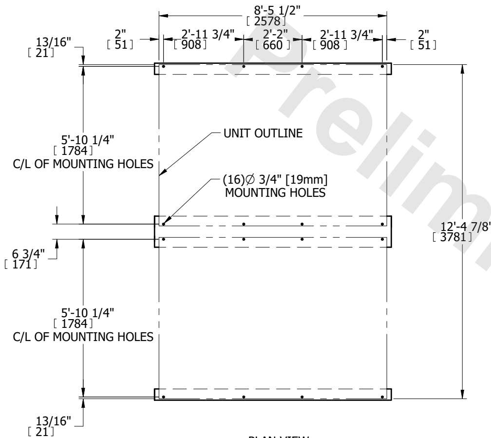
PLAN VIEW
