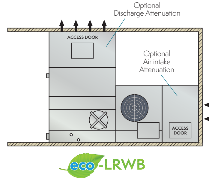
NOTE: eco-LRWB Shown Ducted on Both Inlet and Discharge
