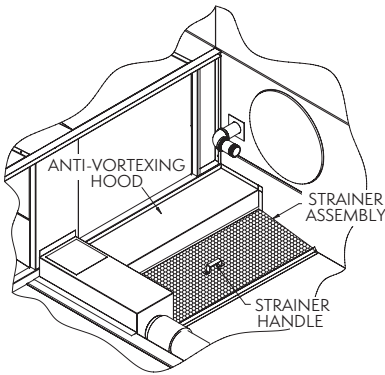
Figure 12 — LRWB/LRC Strainer Assembly
