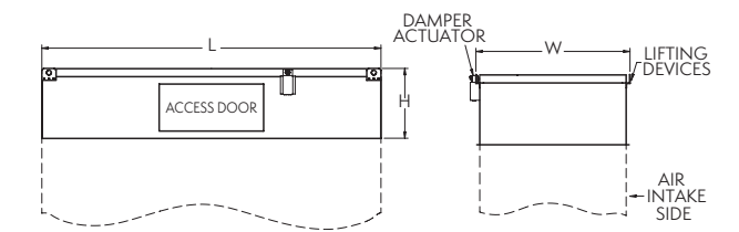
Straight-Sided Discharge Hood (See page 21 for dimensions)
