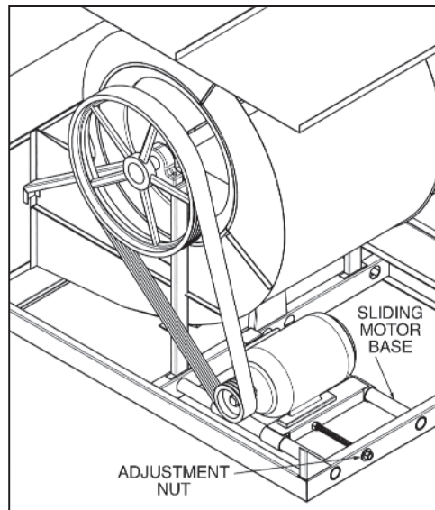
Figure 7 – Externally Mounted Motors, LPT Units
