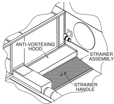
Figure 11 – LPT Strainer Assembly
