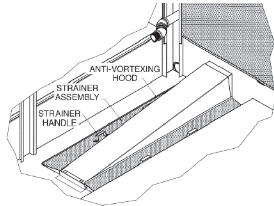
Figure 9 – Dual Strainer Assembly
