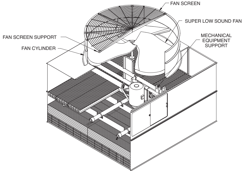
UT 12' Wide Unit with Side Connection Shown
