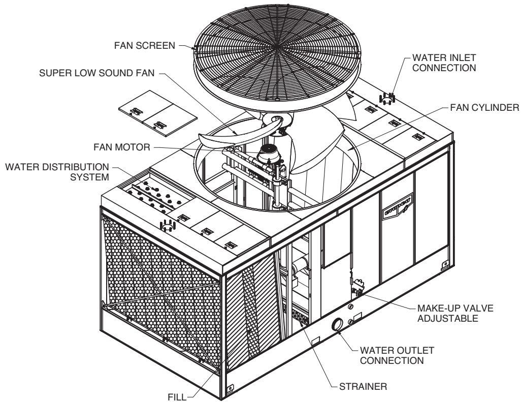
12' Wide Single Stack AXS Unit Shown
