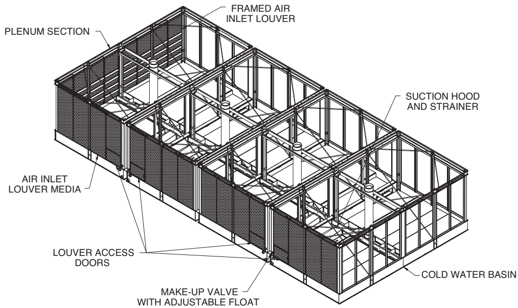
PAN & PLENUM SECTION (FOUR CELLS SHOWN)
