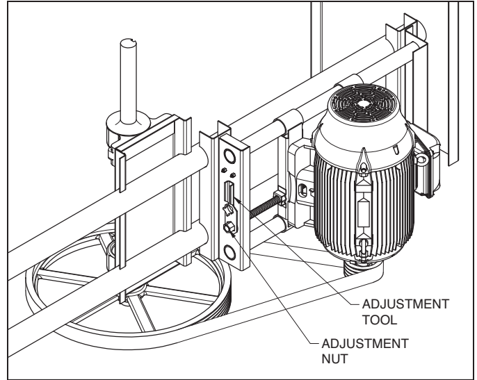
Figure 6 – Internally Mounted Motors, AXS Units
