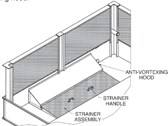
Figure 8 – Single Strainer Assembly
