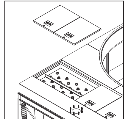
Figure 16 – Hot Water Basins
