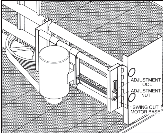
Figure 5 – Internally Mounted Motors, AT/UT/USS Units
