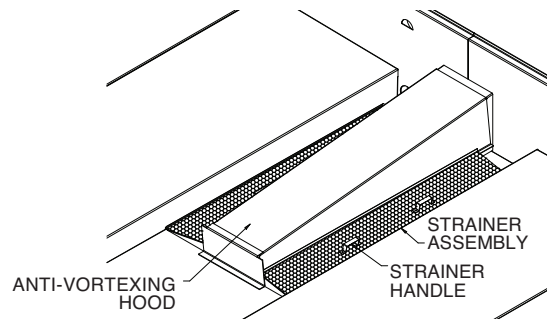
Figure 12 – AXS Strainer Assembly
