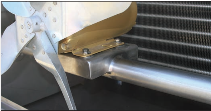
Fully Welded Stainless Pipe Motor Mount with "Spacer" Between the Motor and the Support for Complete Cleaning
